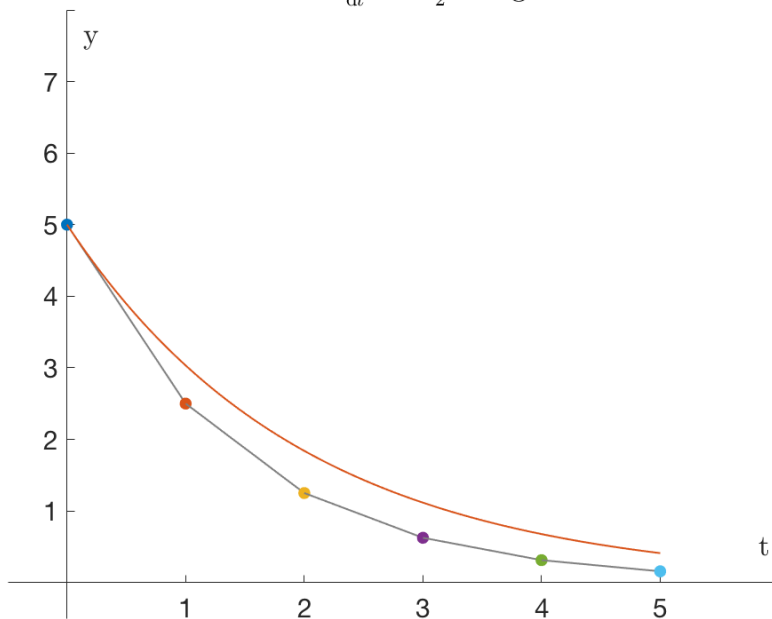
Numerical solution to \frac{dy}{dt} = -\frac{y}{2} using Euler's Method
